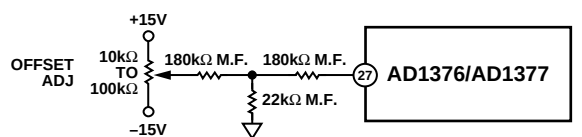
Figure 7. Low Temperature Coefficient Zero Adjustment Circuit
