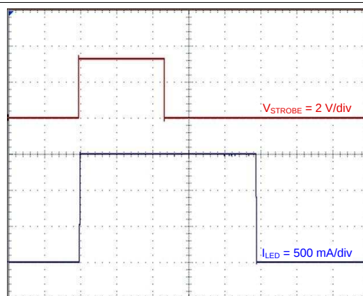
Figure 60. Edge-Sensitive Strobe
