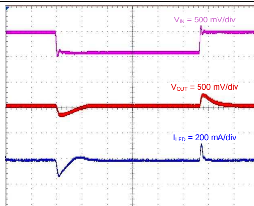
Figure 44. Line-step (400 mV) During Flash
