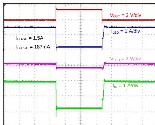
Figure 48. TX-Mask Event, Default Settings
