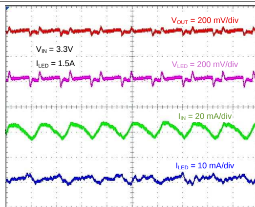
Figure 46. LED Current Ripple
