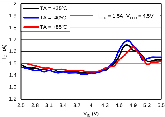
Figure 8. Inductor Current vs. Input Voltage, CL = 1.3 A
