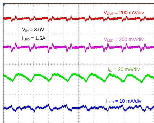
Figure 45. LED Current Ripple
