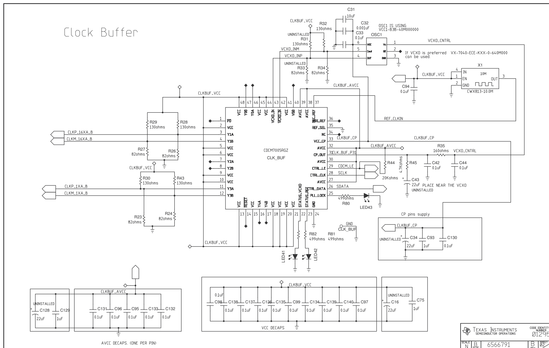
Figure 19. Schematic 2 of 10
