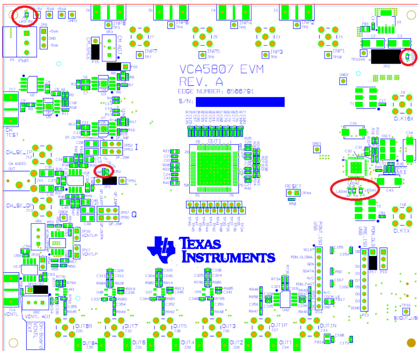
Figure 8. PCB Layout With Jumper Positions
