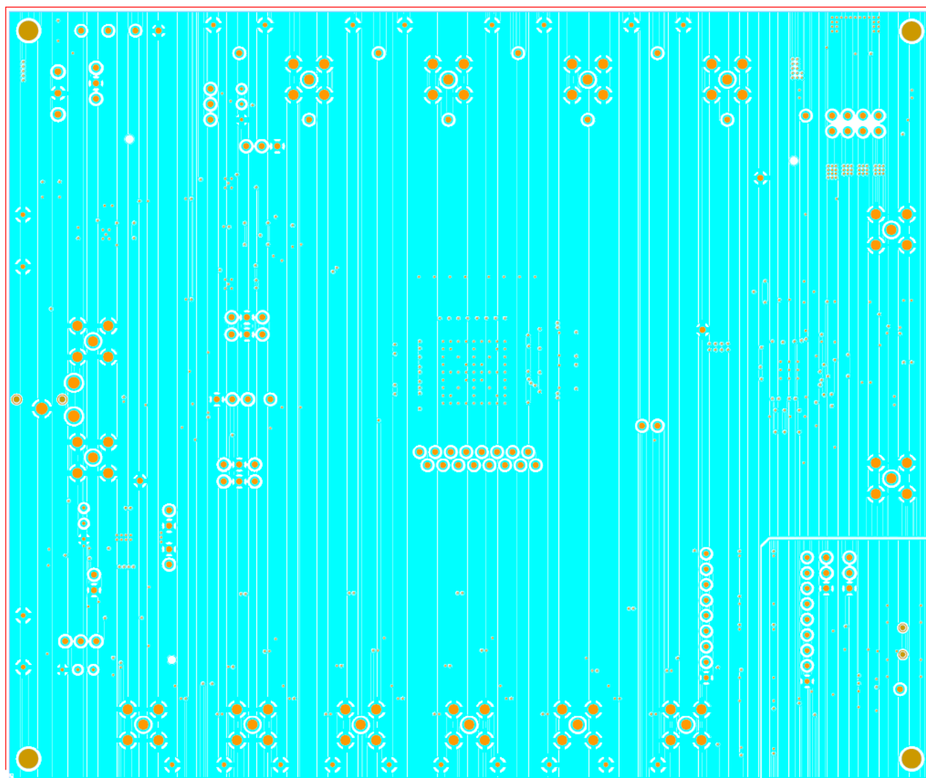
Figure 16. Fifth Layer - Ground
