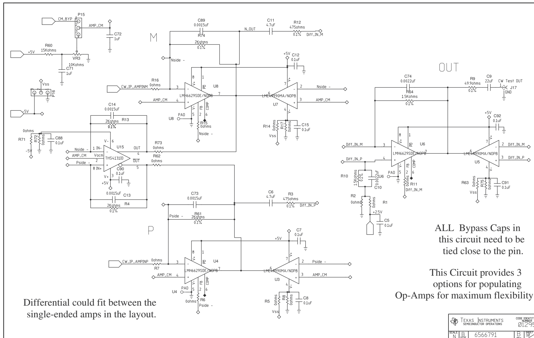
Figure 27. Schematic 10 of 10
