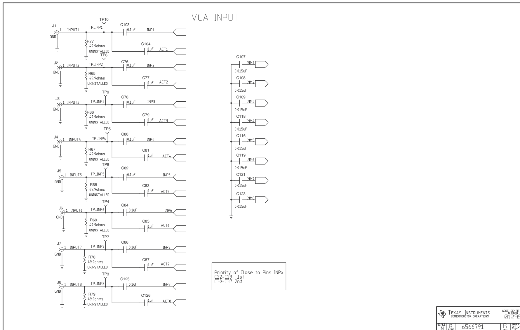
Figure 20. Schematic 3 of 10
