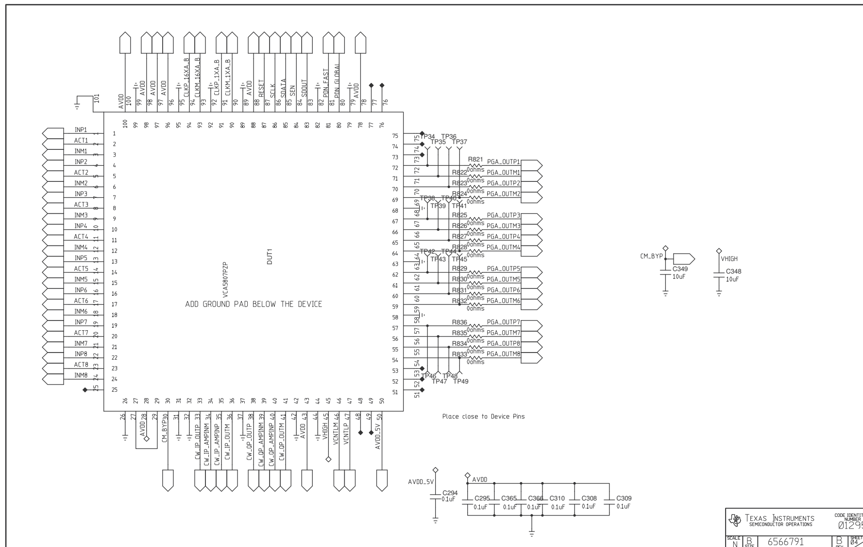
Figure 21. Schematic 4 of 10
