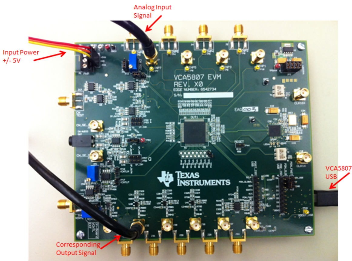
Figure 7. HW Setup
