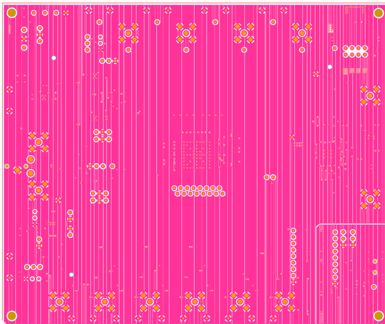
Figure 13. Second Layer - Ground
