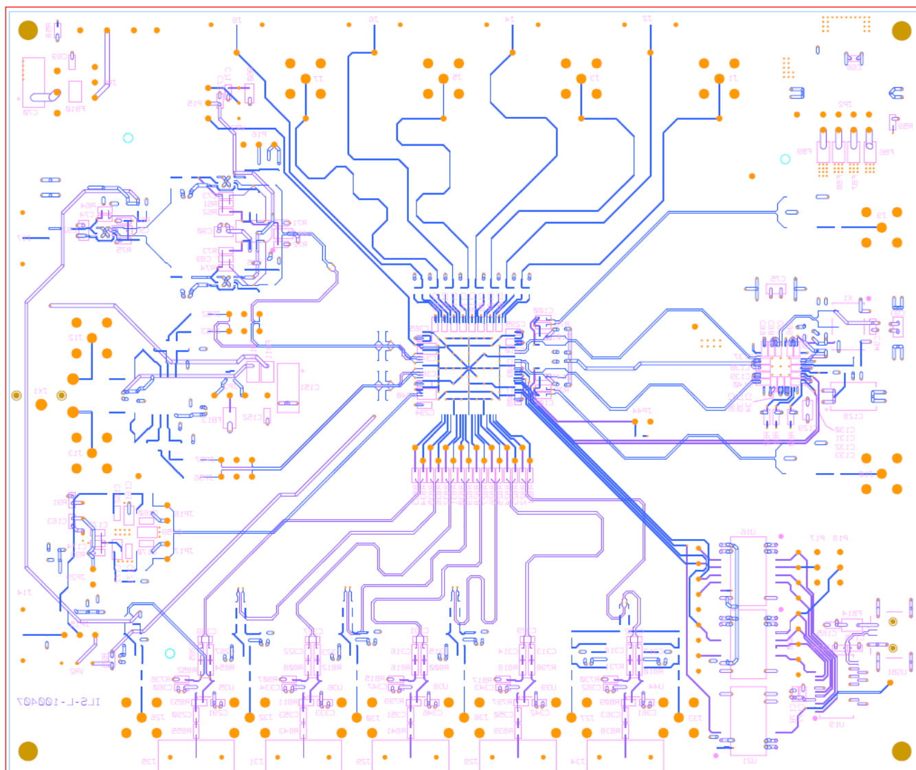
Figure 17. Bottom Layer - Signal
