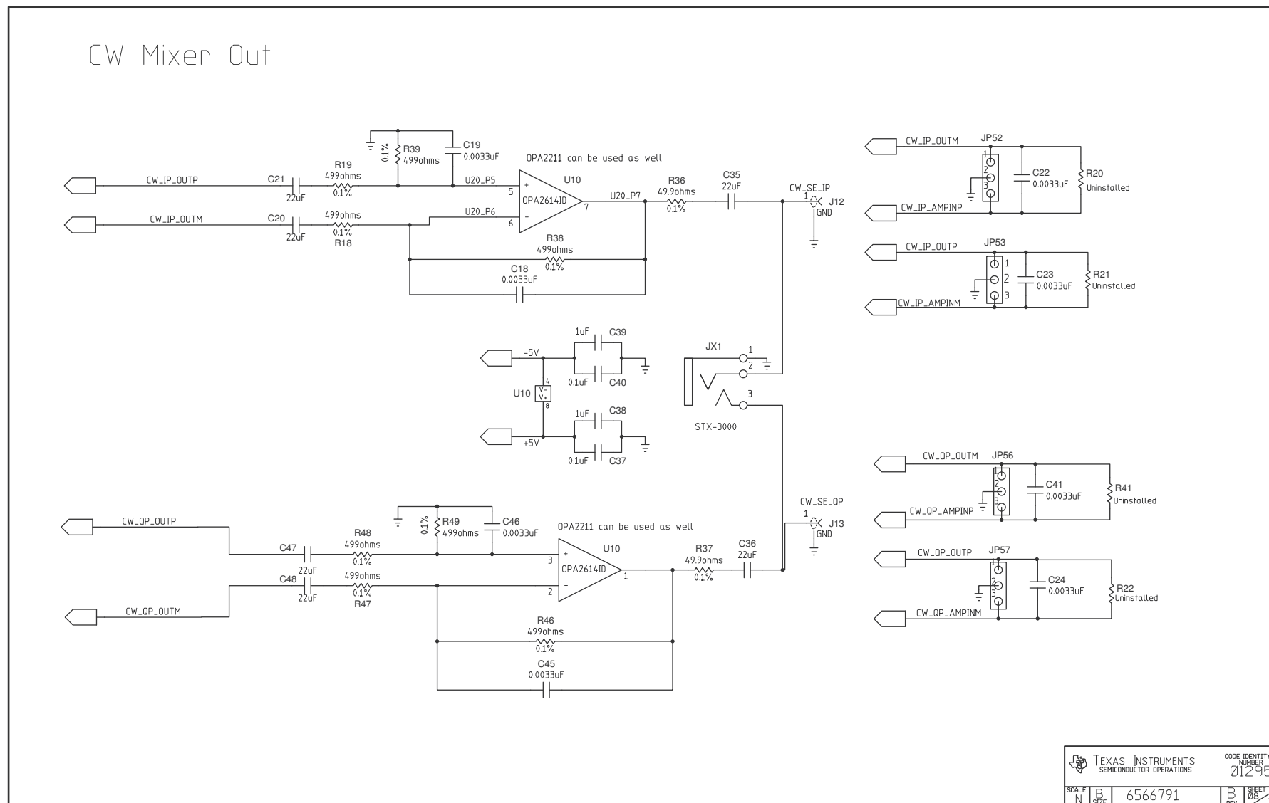
Figure 25. Schematic 8 of 10
