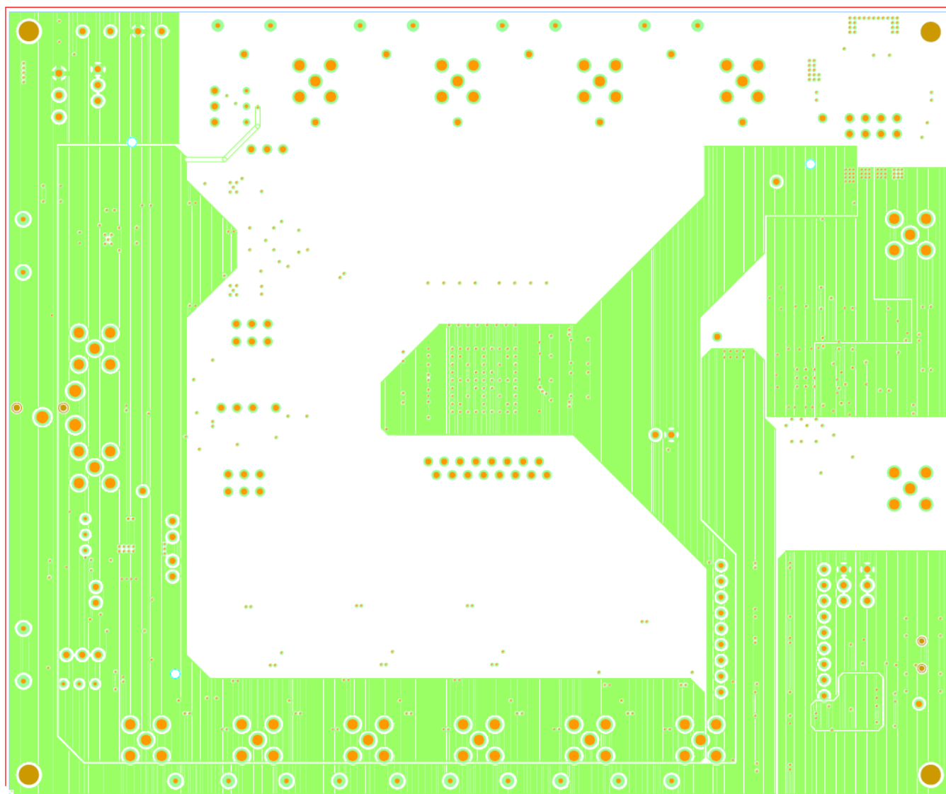
Figure 14. Third Layer - Power
