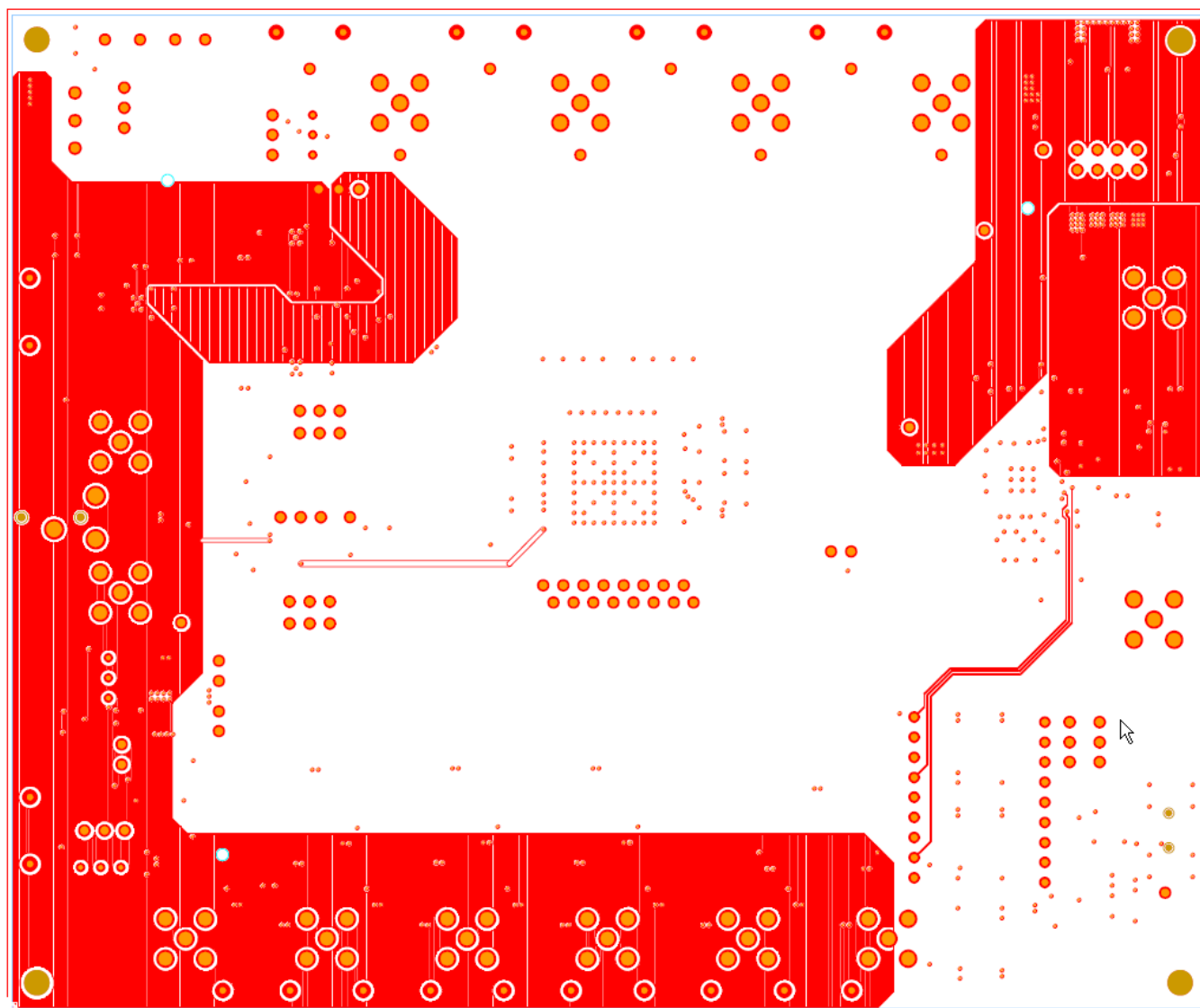
Figure 15. Fourth Layer - Signal
