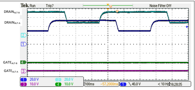
Figure 127. 4-Pair Open Circuit Detection Signature
