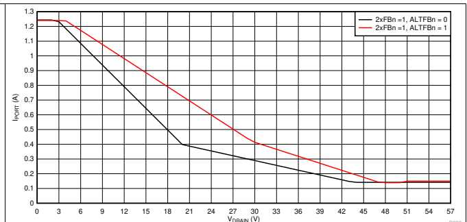
Figure 112. 2x Mode (2xFBn = 1) Foldback Curves, I PORT vs V DRAIN
