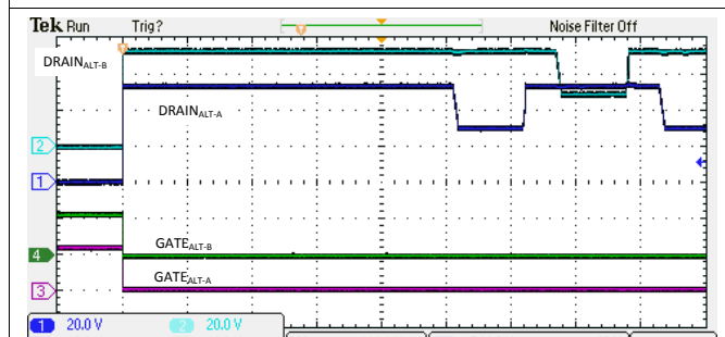
Figure 124. 4-Pair Backoff Due to 4PPCut Fault
