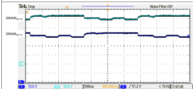
Figure 128. 4-Pair Low Resistance (11kΩ) Detection Signature
