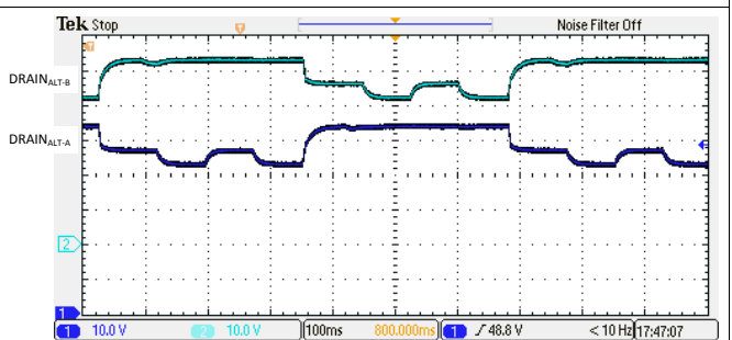
Figure 129. 4-Pair High Resistance (36kΩ) Detection Signature
