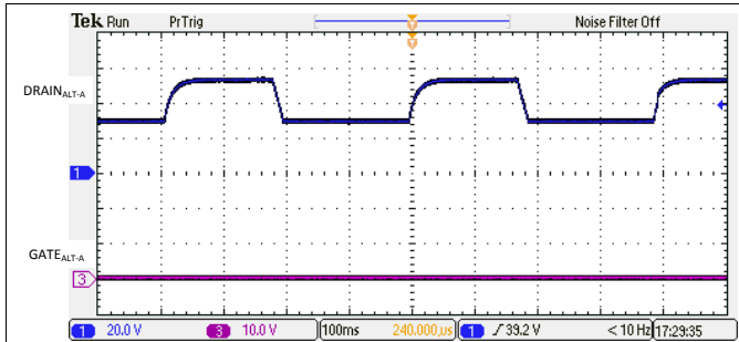
Figure 126. 2-Pair Open Circuit Detection Signature
