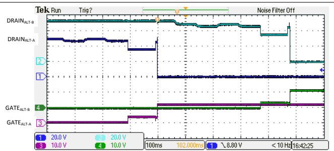
Figure 141. 4-Pair Dual Signature 1-Finger Classification and Turn On
