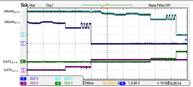
Figure 143. 4-Pair Dual Signature 4-Finger Classification and Turn On
