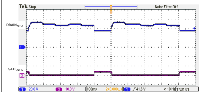
Figure 130. 2-Pair Semi-Auto Mode Discovery with a Valid Class 0-3 Load
