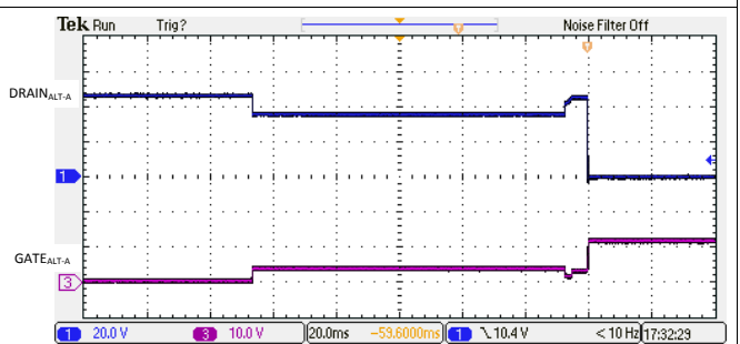
Figure 131. 2-Pair 1-Finger Classification and Turn On
