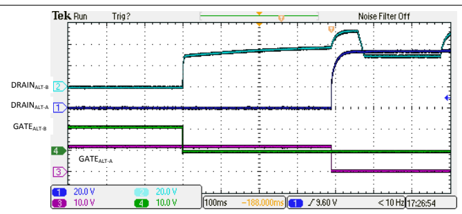
Figure 125. 4-Pair Single Signature Class 0-4 Disconnect
