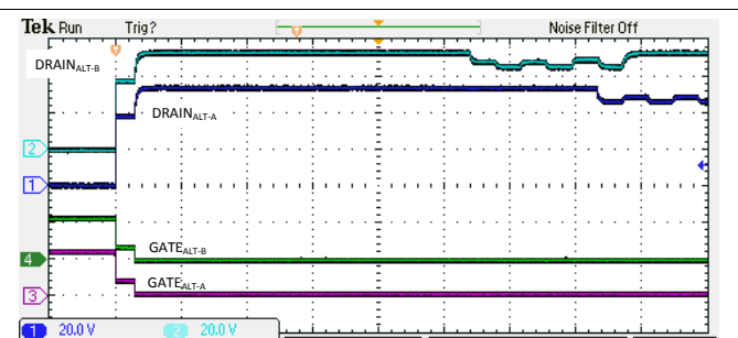
Figure 123. 4-Pair Backoff Due to I_{LIM} Fault
