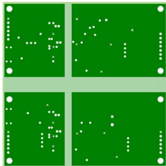
Figure 20. Layer 3: Power Plane
