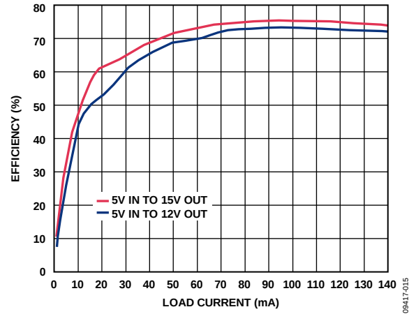
Figure 15. Double Supply Efficiency with the Coilcraft Transformer for Different Output Options at 500 kHz
