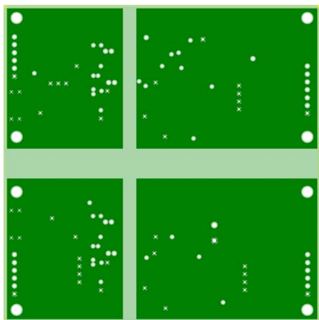
Figure 19. Layer 2: Ground Plane
