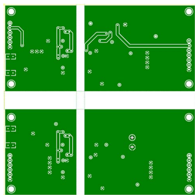
Figure 21. Bottom Layer: Ground Fill
