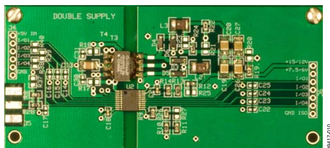
Figure 10. Double Supply
