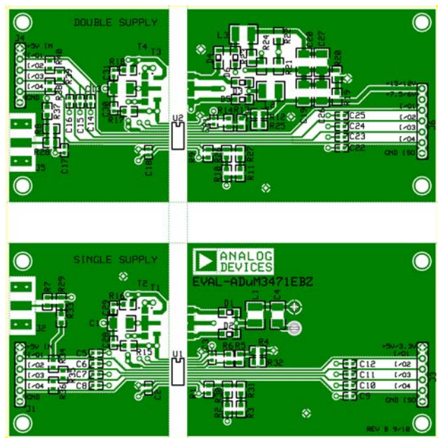
Figure 18. Top Layer: Power Fill
