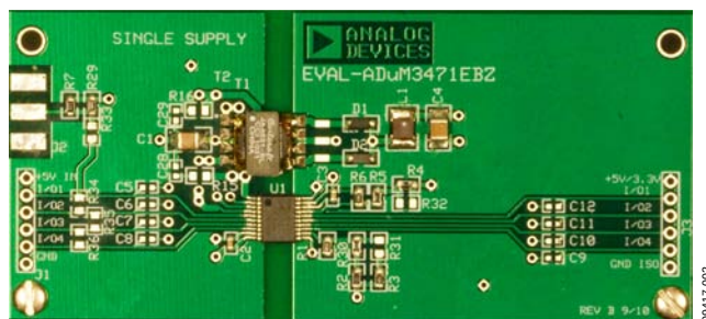
Figure 2. Single Supply
