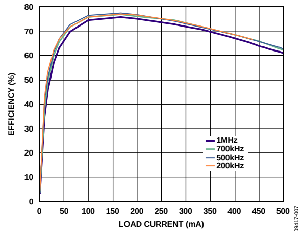
Figure 7. 5 V In to 5 V Out Efficiency with the Halo Transformer at Various Switching Frequencies
