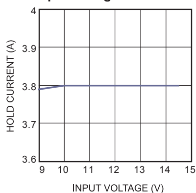
Hold Current vs. Input Voltage
