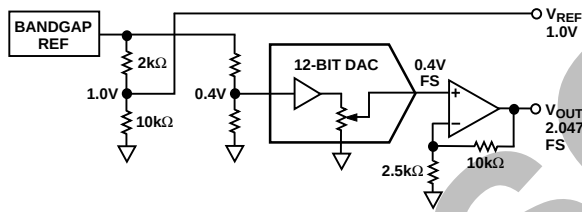
Figure 22. AD8303 Equivalent Schematic of Analog Section
