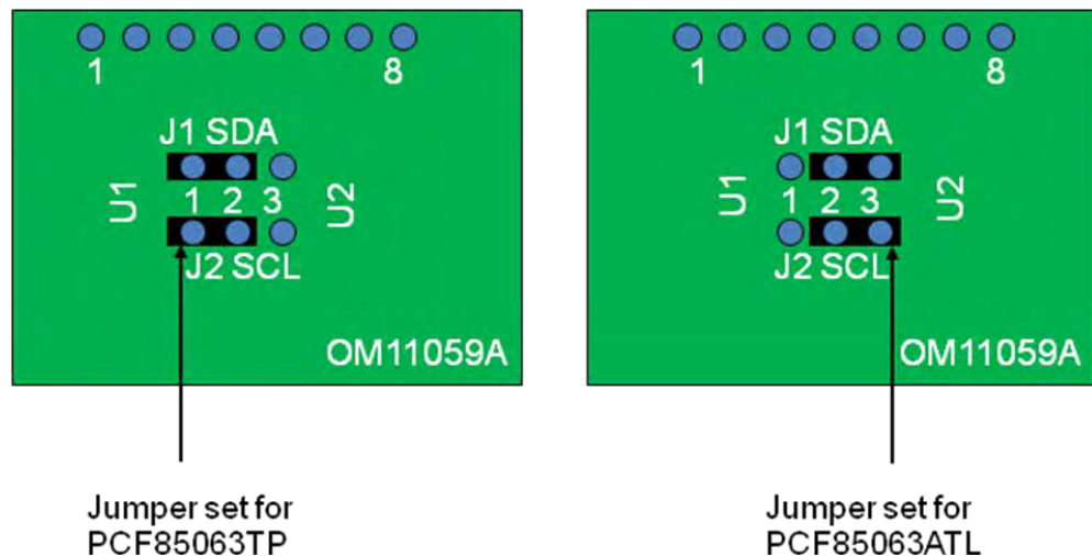
Fig 5. Jumper settings
