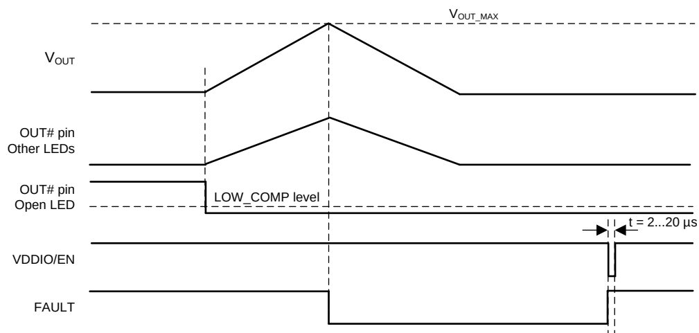
Figure 15. LED Open Fault
