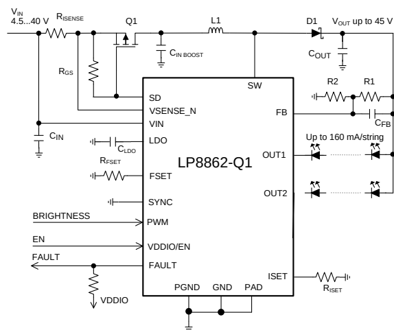
Simplified Schematic
