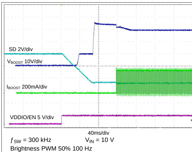
Figure 20. Typical Start-Up
