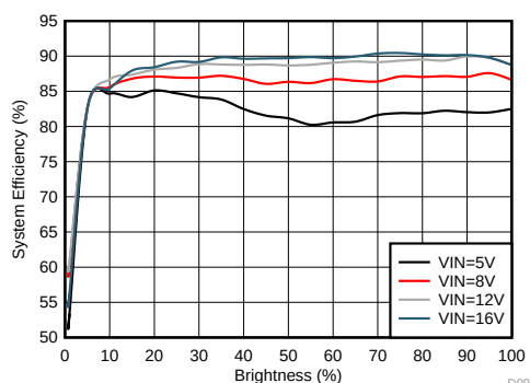
System Efficiency
