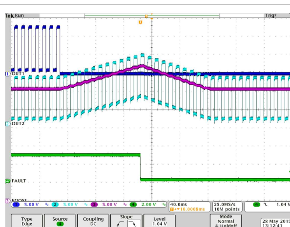
Figure 21. Open LED Fault
