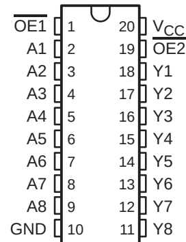
SN54LVTH540 . . . J OR W PACKAGE SN74LVTH540 . . . DB, DW, NS, OR PW PACKAGE (TOP VIEW)
