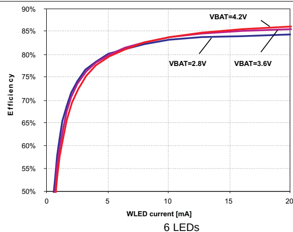
Figure 34. Efficiency
