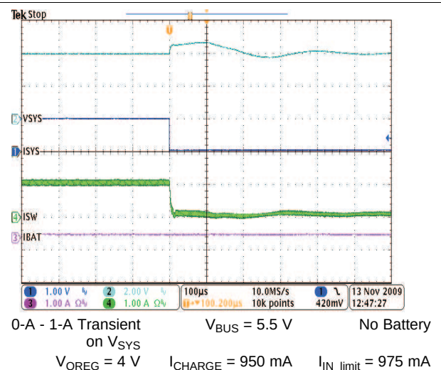
Figure 59. Transient Response
