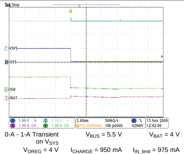
Figure 57. Transient Response
