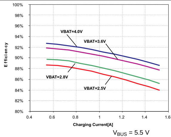
Figure 8. Charger Efficiency
