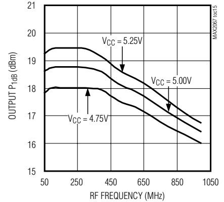
OUTPUT P_{1dB} vs. RF FREQUENCY
