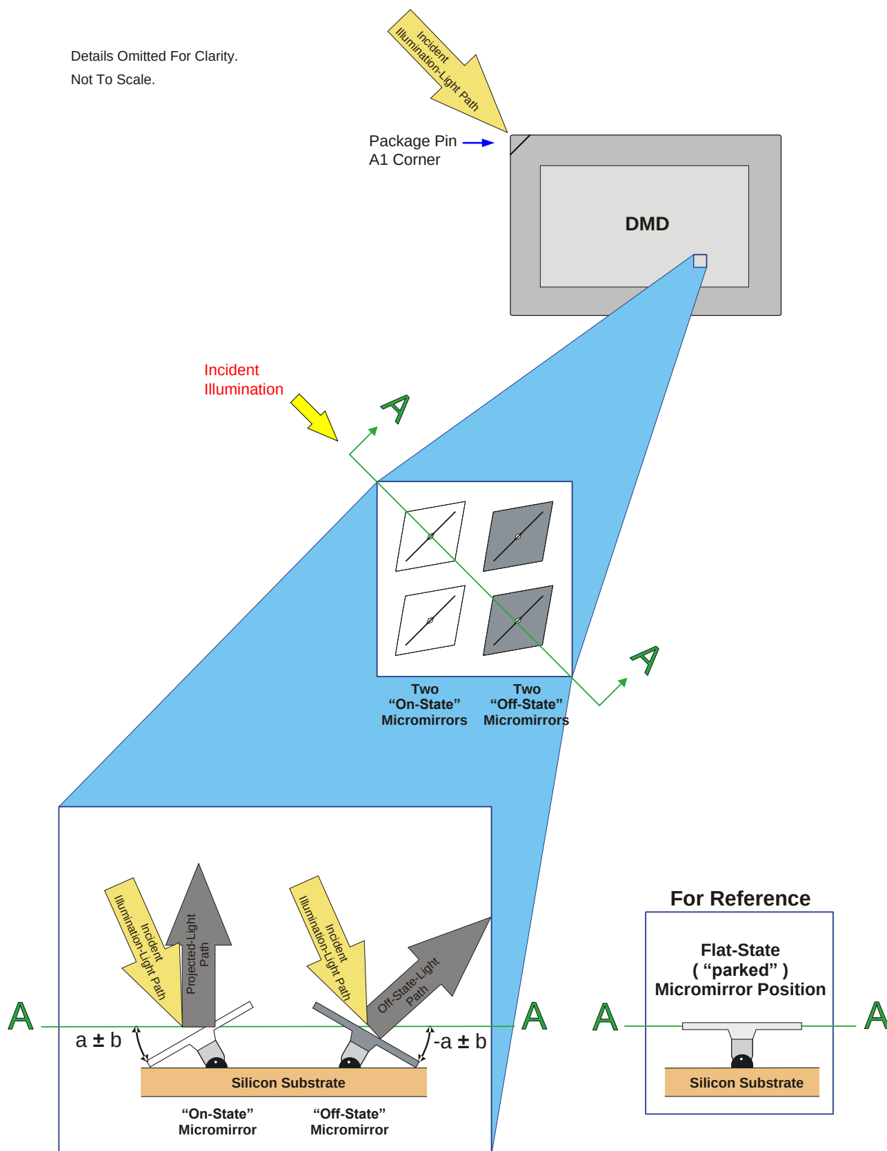
Figure 15. Micromirror Landed Positions and Light Paths
