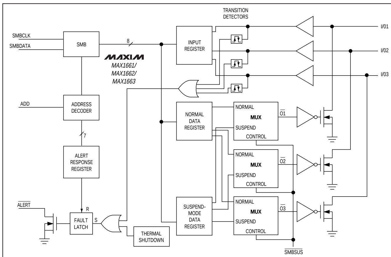
Figure 1. Functional Diagram
