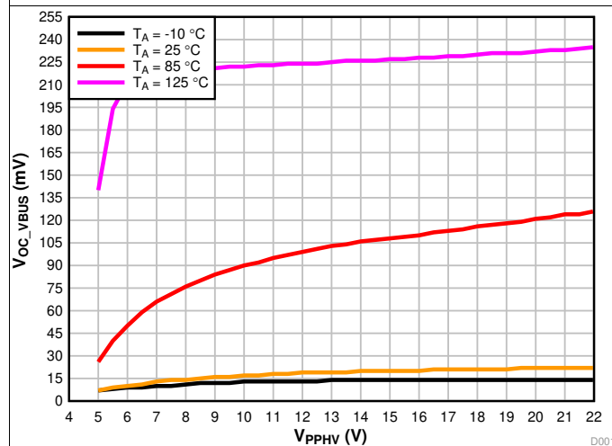
Figure 5. V_{OC\_VBUS} , VBUS Open Circuit Voltage versus PPHV
