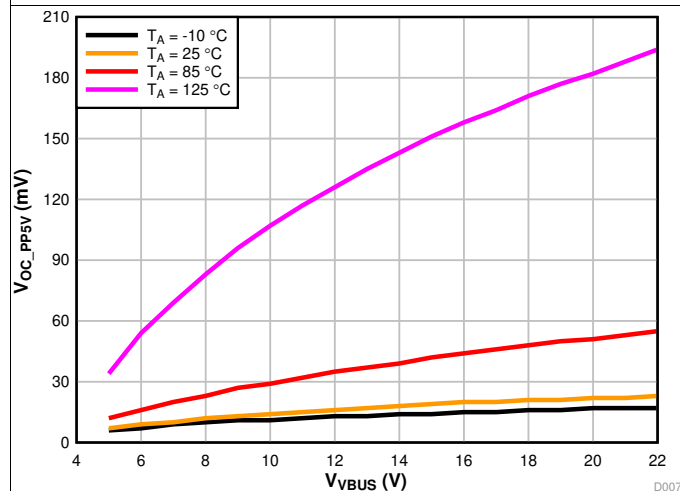
Figure 3. V_{OC\_PP5V} , PP5V Open Circuit Voltage versus VBUS
