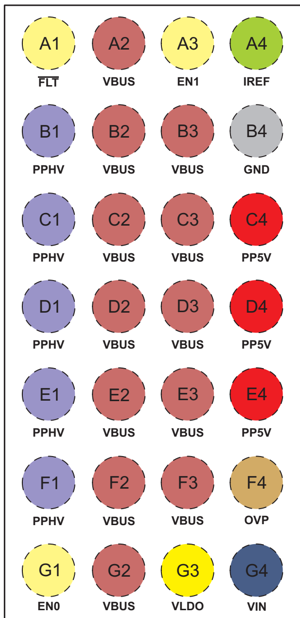
Pin Functions
