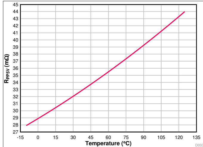
Figure 1. R_{PP5V} versus Temperature
