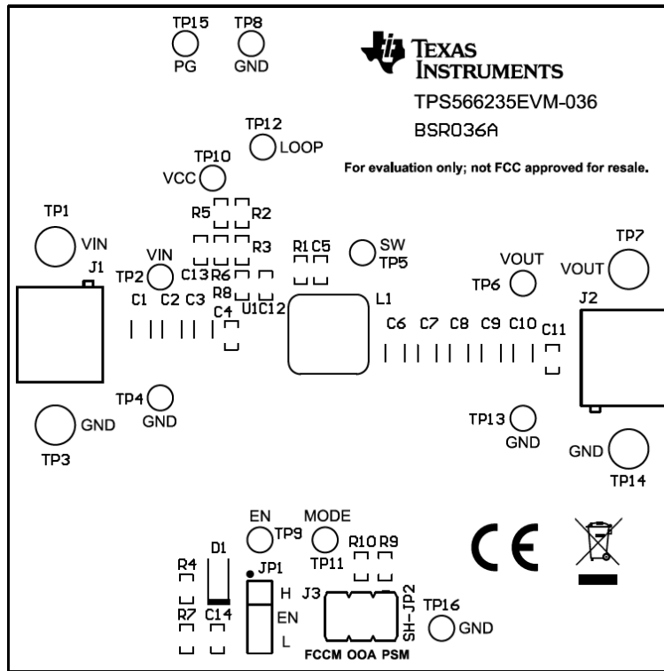
Figure 2. Component Placement (Top Layer)
