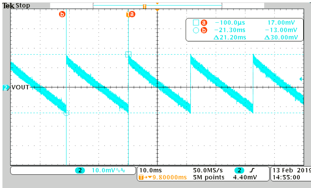
Figure 11. V_{OUT} Ripple with 0-A Loading
