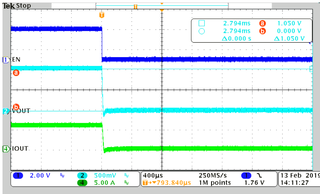
Figure 10. Power Down with 6-A Loading Controlled by EN Pin
