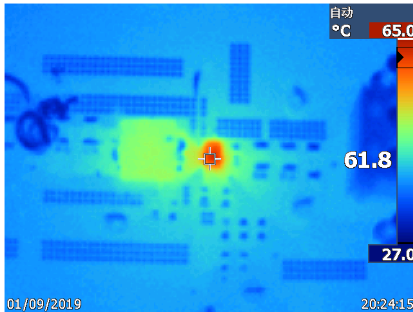
Figure 15. Thermal Information at 6-A Full Loading
