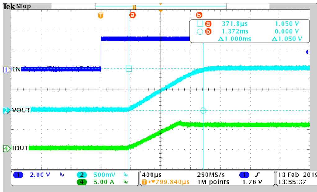
Figure 9. Power up with 6 A loading controlled by EN pin
