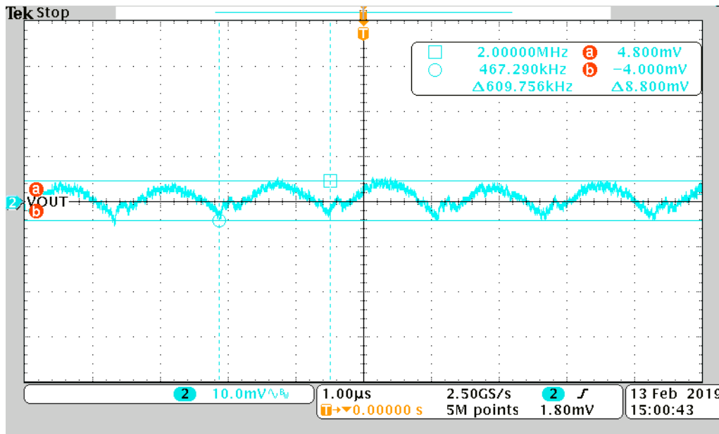
Figure 12. V_{OUT} Ripple with 6-A Loading
