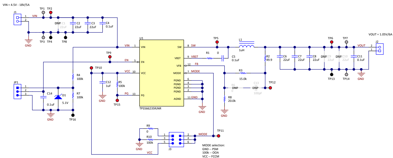
Figure 1. TPS566235EVM-036 Evaluation Module Schematic
