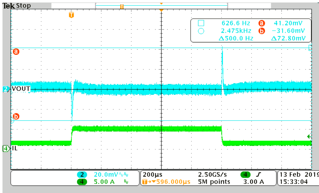
Figure 14. Load Transient Response from 1.2 A to 4.8 A with R6 = 0 Ω and C13 = 100 pF
