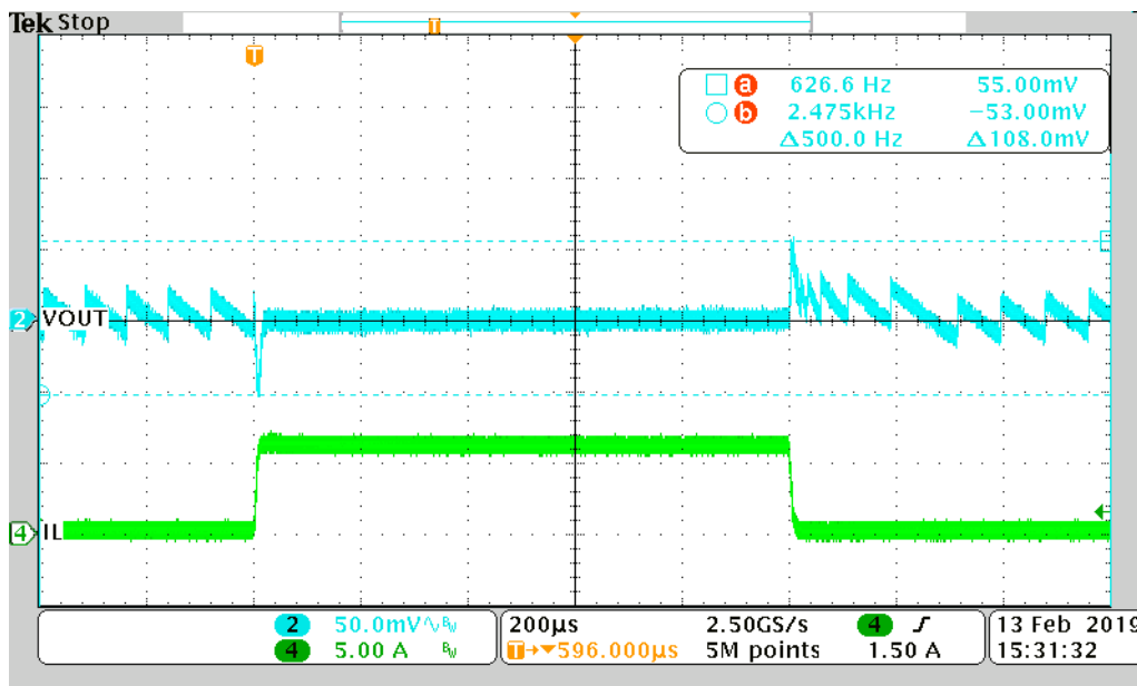
Figure 13. Load Transient Response from 0 A to 6 A with R_6 = 0 \Omega and C_{13} = 100 \text{ pF}
