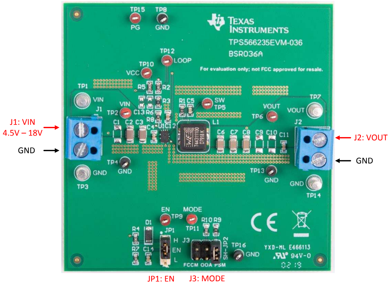
Figure 7. Connectors and Jumpers Placement (Top View)
