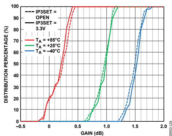
Figure 26. Gain
