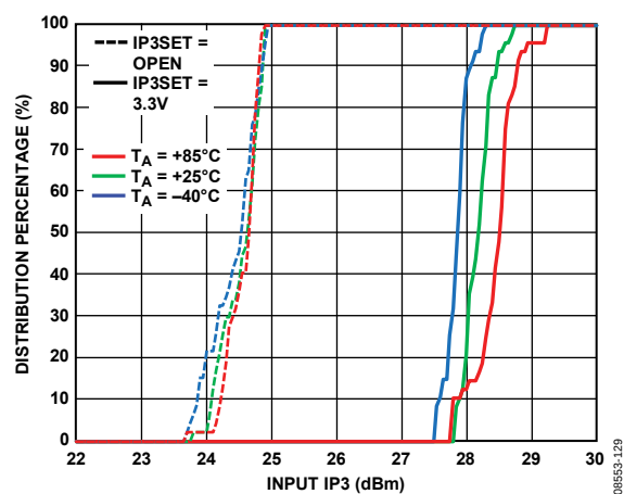
Figure 29. Input IP3
