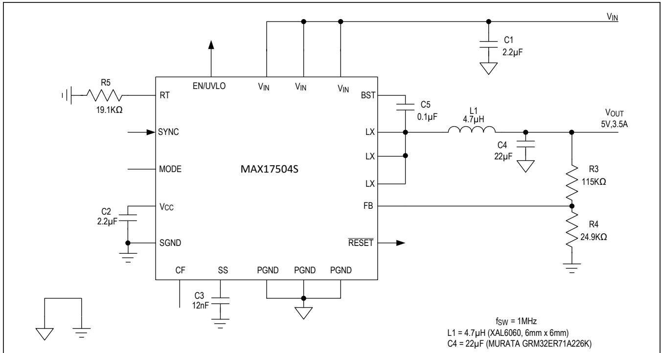
Figure 5. MAX17504S Typical Operating Circuit for 5V Output, 1MHz Switching Frequency
