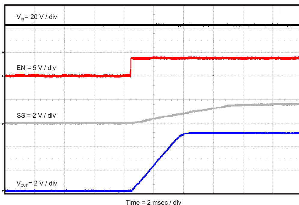
Figure 12. TPS54336AEVM-010 Start-up Relative to Enable
