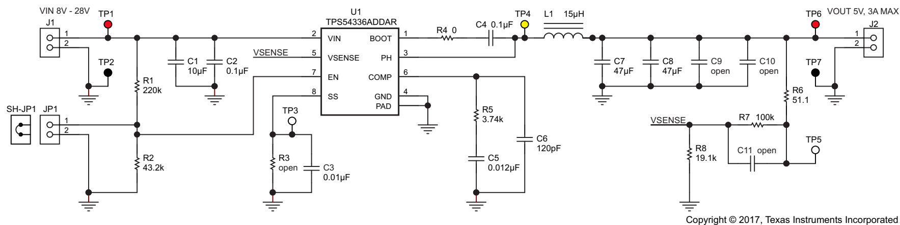
Figure 18. TPS54336AEVM-010 Schematic
