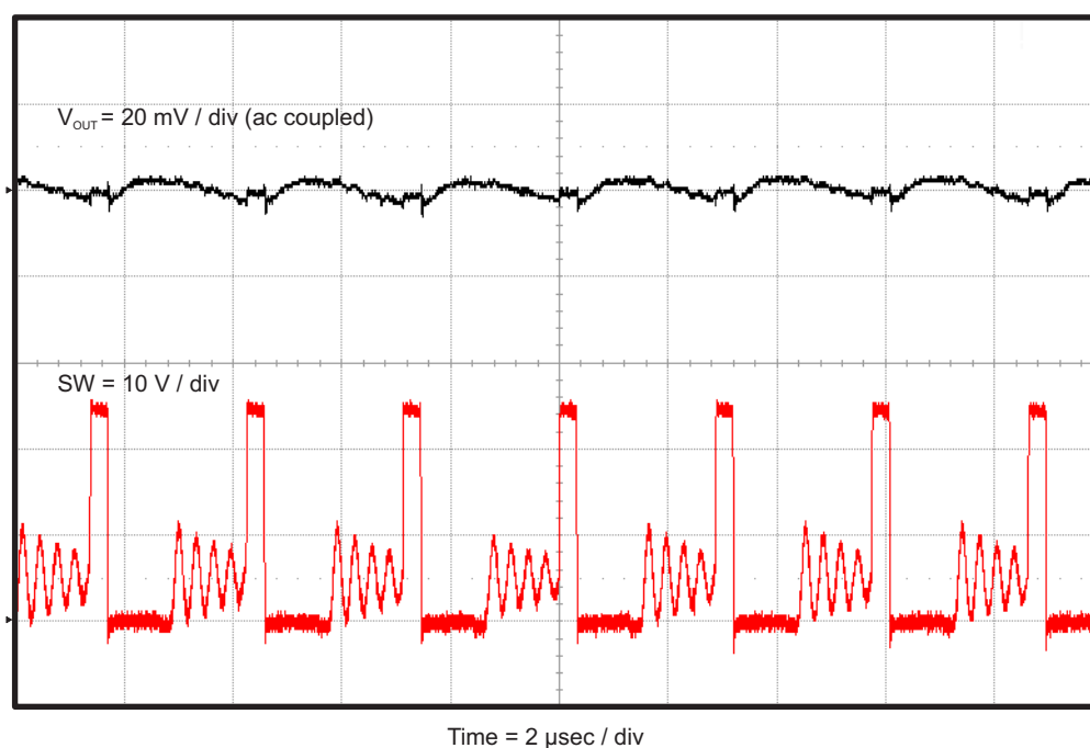
Figure 8. TPS54336AEVM-010 Output Ripple, I_{OUT} = 100 mA
