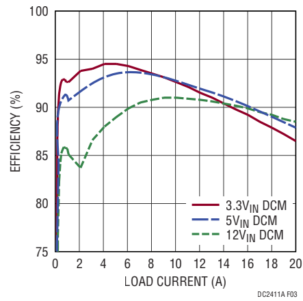
Figure 3. Efficiency vs Load Current ( V_O = 1.2V , 400kHz)
