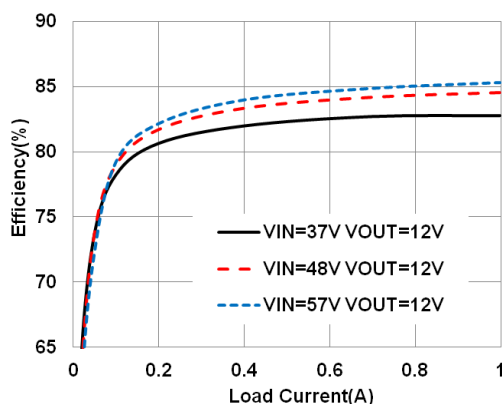
Efficiency vs. Load Current V_{IN} = 37V, 48V , and 57V , V_{OUT} = 12V
