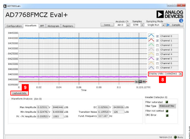
Figure 20. Waveform Tab
