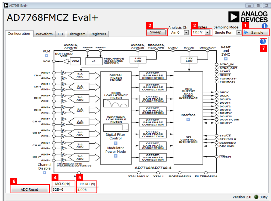
Figure 17. Evaluation Software Main Window
