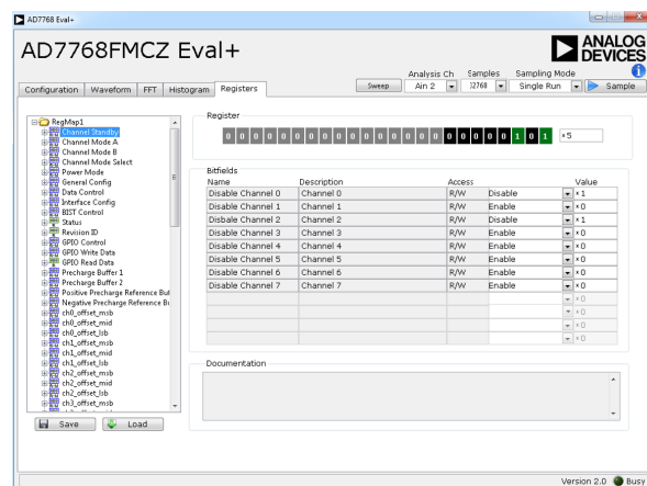
Figure 23. Registers Tab
