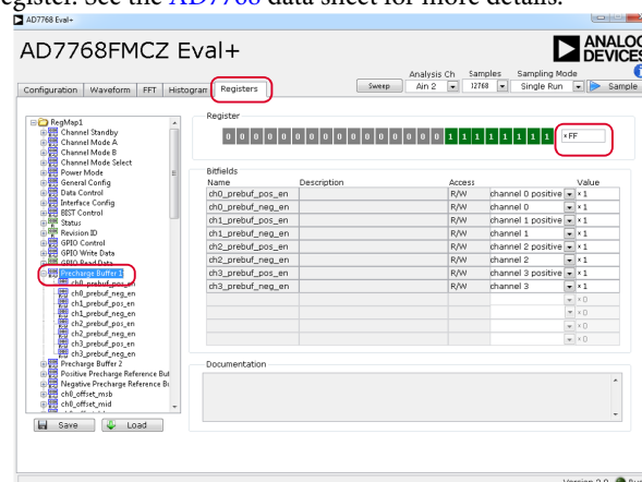
Figure 24. Enabling/Disabling the Precharge Buffers
