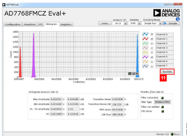
Figure 22. Histogram Tab
