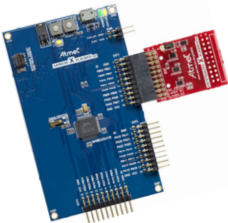
Figure 2. CryptoAuthXplained PRO Daughterboard on an Atmel Xplained Development Board
