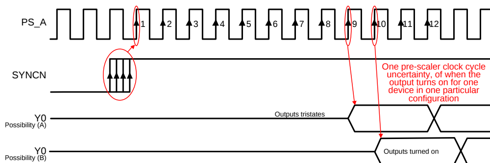
Figure 48. SYNCN to Output Delay Uncertainty
