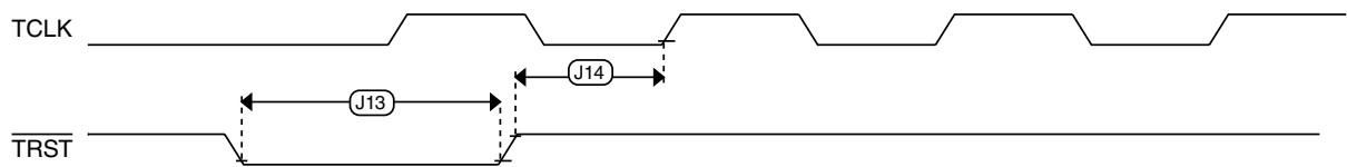
Figure 33. TRST timing
