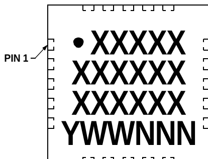
20-Lead QFN (4x4x0.9 mm)
