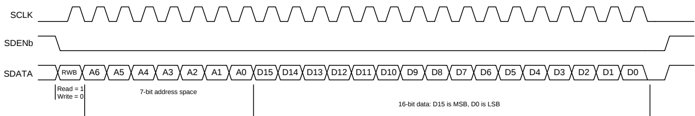
Figure 62. Serial Register Write Timing Diagram
