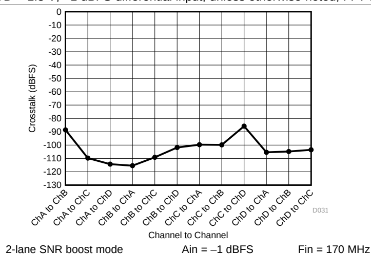
Figure 36. SNR Boost Crosstalk by Channel
