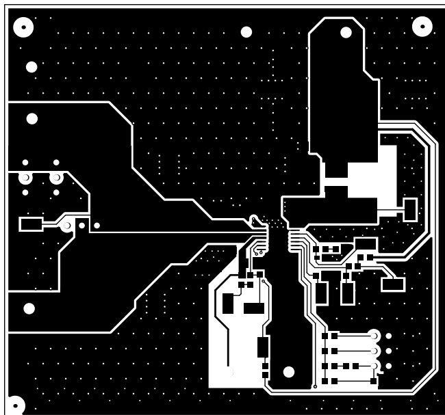
Figure 4. Layout—Top
