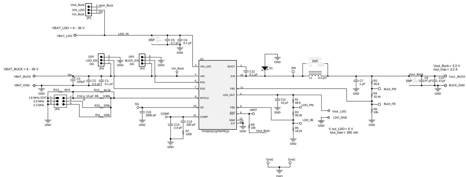
Figure 1. TPS65321-Q1 Schematic
