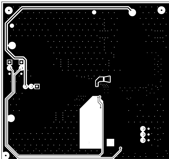
Figure 5. Layout—Bottom
