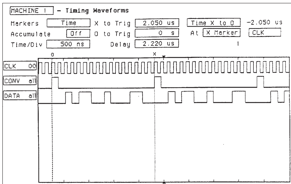
Logic Analyzer Waveforms Show 2.05 \mu s Throughput Rate (Input Voltage = 1.606V, Output Code = 0110 0100 0110 = 1606 10 )
