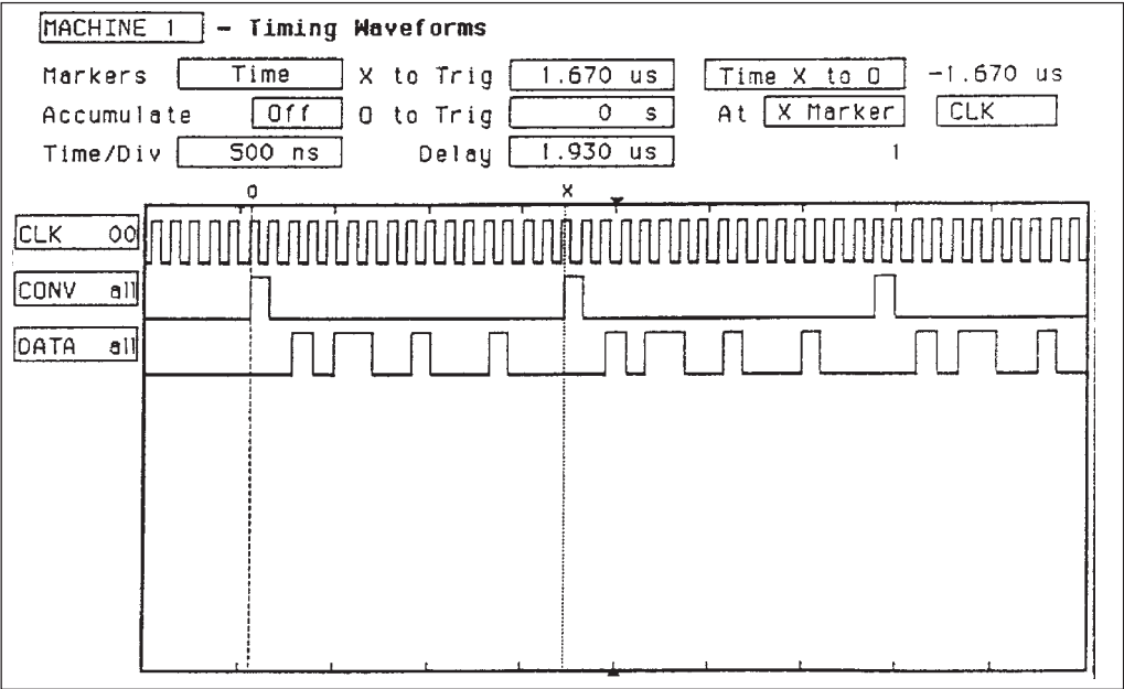
Logic Analyzer Waveforms Show 1.67µs Throughput Rate (Input Voltage = 1.604V, Output Code = 0110 0100 0100 = 1604 10 )
