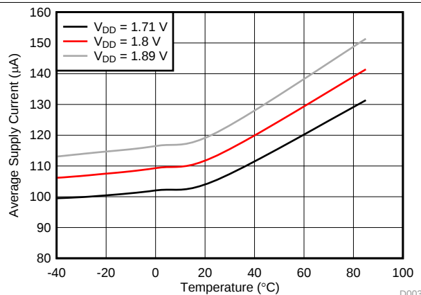
Figure 5. Supply Current vs Temperature. Sensor R_P = 650\text{ }^{\circ}\Omega , Scan Rate = 40 SPS.
