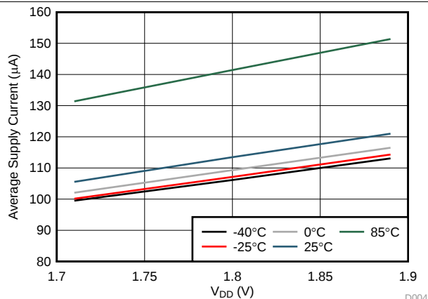
Figure 6. Supply Current vs V_{DD} . Sensor R_P = 650\text{ }^{\circ}\Omega , Scan Rate = 40 SPS.
