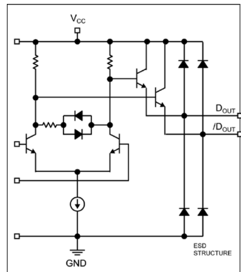
Figure 3. Output Structure
