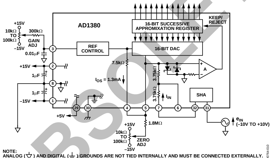
Figure 10. Analog and Power Connections for Bipolar -10\text{ V} to +10\text{ V} Input Range
