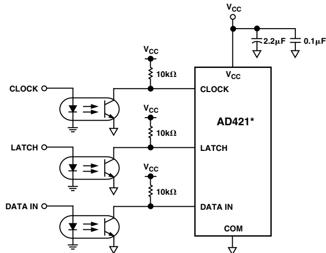
Figure 10. Opto-Isolated Interface
