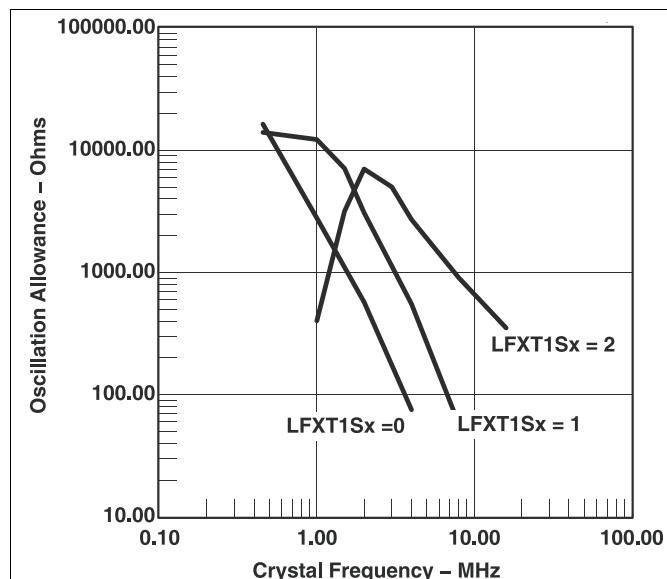
Figure 4-24. Oscillation Allowance vs Crystal Frequency, C_{L,eff} = 15 pF, T_A = 25^\circ\text{C}
