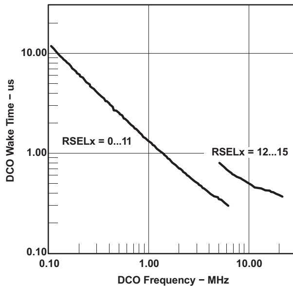
Figure 4-19. Clock Wake-Up Time From LPM3 vs DCO Frequency
