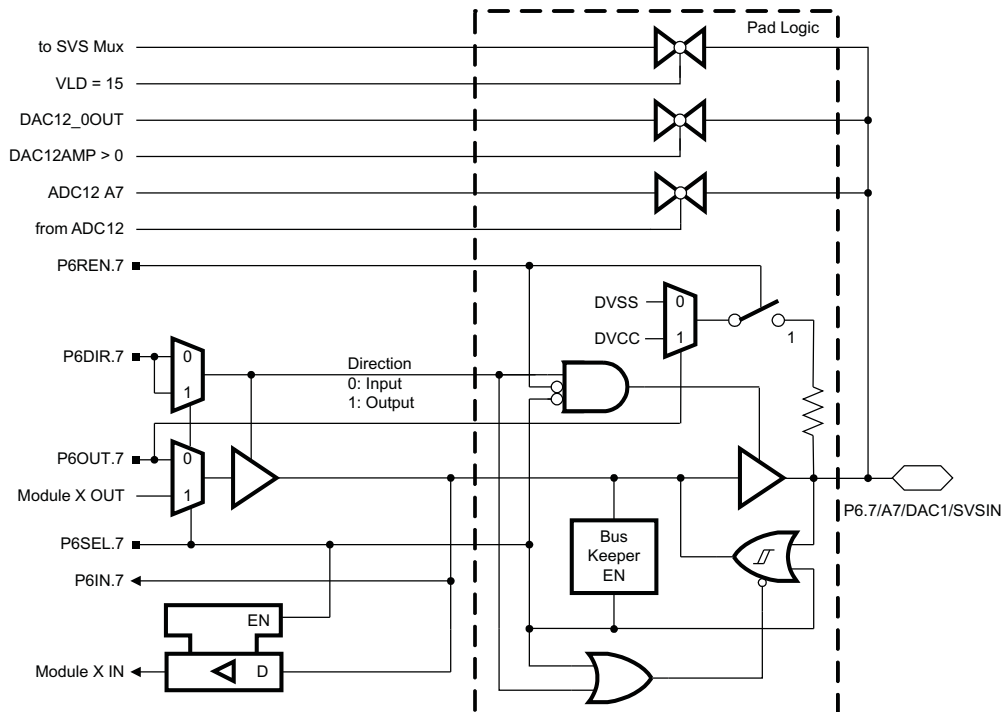
Figure 6-9. Port P6 (P6.7) Pin Schematic
