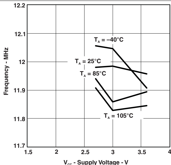
Figure 4-17. Calibrated 12-MHz DCO Frequency vs V_{CC}
