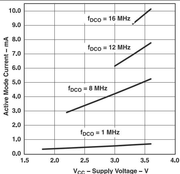
Figure 4-3. Active-Mode Current vs V_{CC} , T_A = 25^\circ\text{C}
