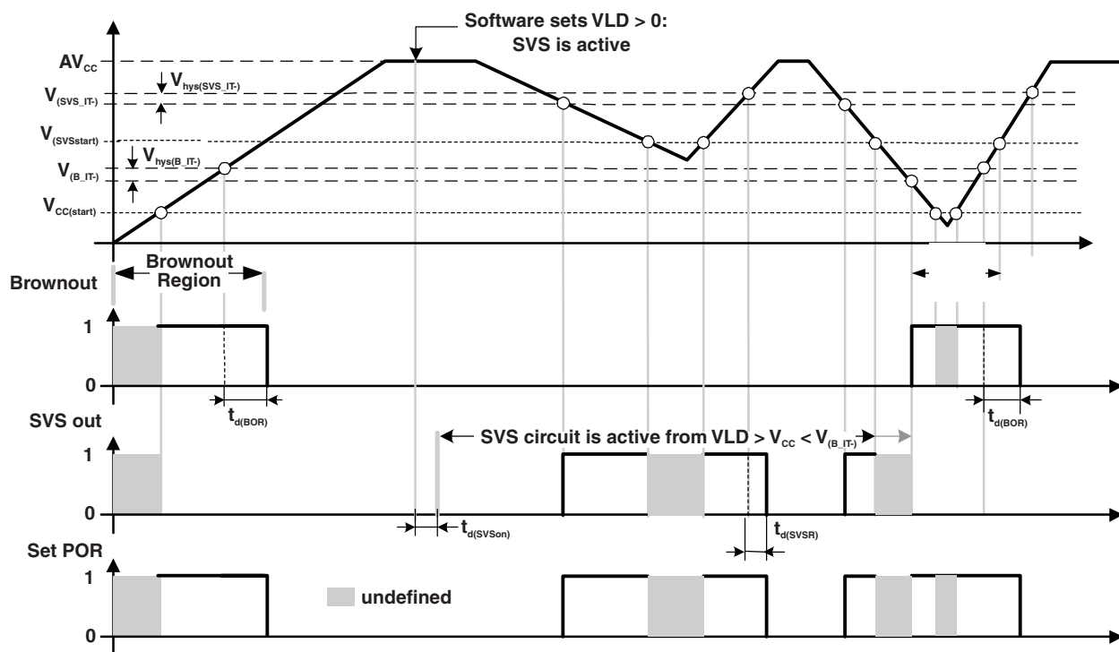
Figure 4-13. SVS Reset (SVSR) vs Supply Voltage
