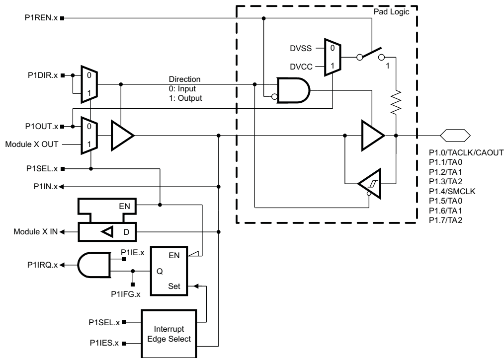
Figure 6-1. Port P1 (P1.0 to P1.7) Pin Schematic
