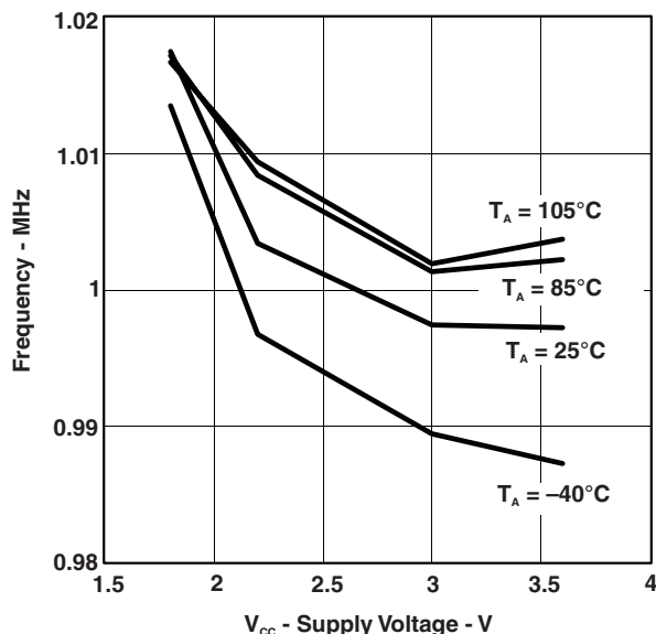
Figure 4-15. Calibrated 1-MHz DCO Frequency vs V_{CC}
