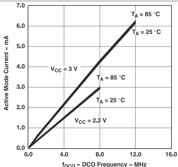
Figure 4-4. Active-Mode Current vs DCO Frequency
