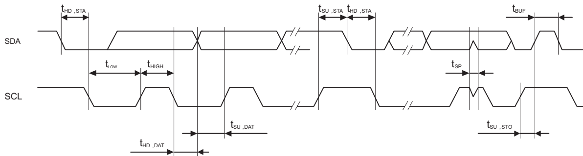
Figure 4-32. I2C Mode Timing
