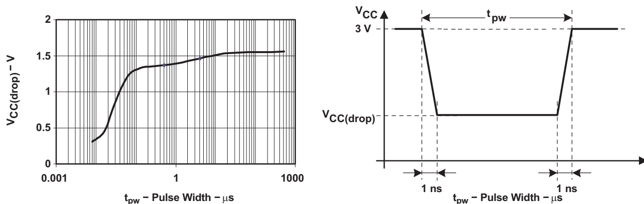
Figure 4-11. V_{CC(drop)} Level With a Square Voltage Drop to Generate a POR/Brownout Signal
