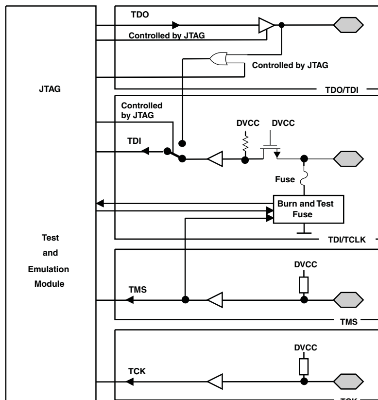
Figure 6-14. JTAG Module
