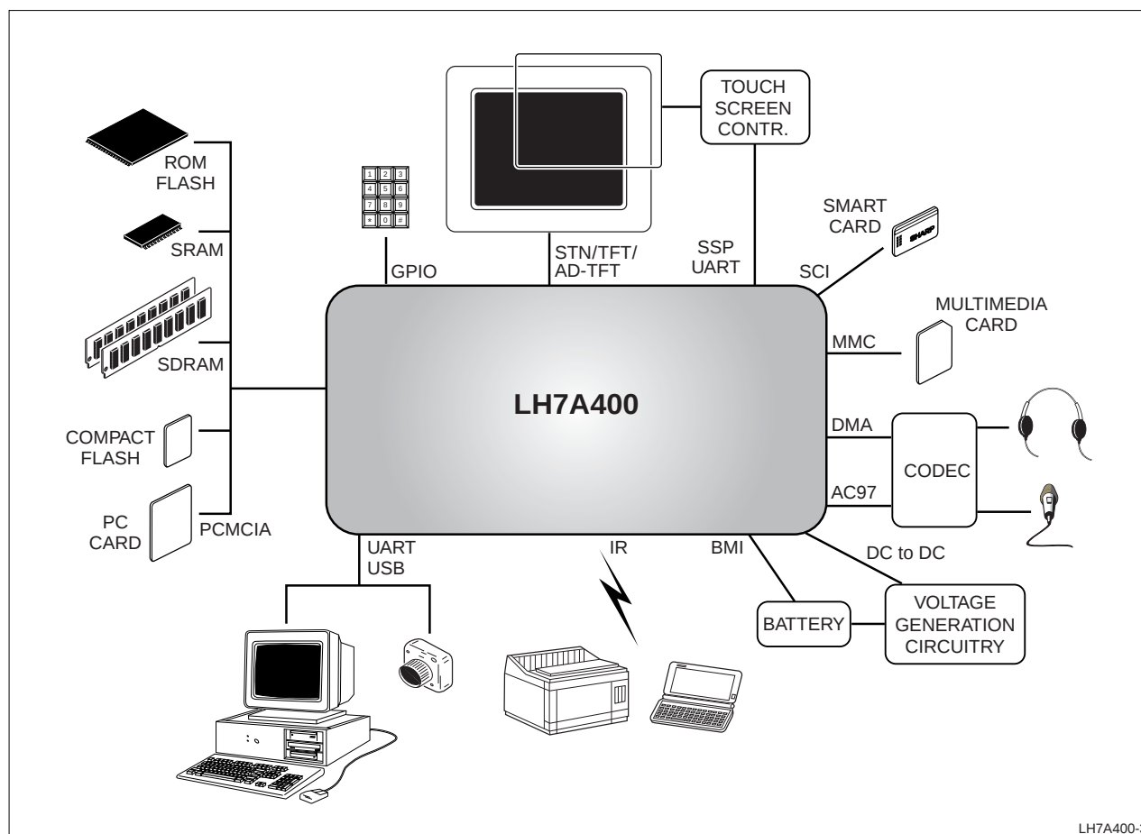
Figure 4. Application Diagram
