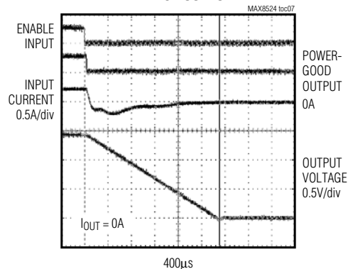
SOFT-STOP WAVEFORMS AT 1.45V OUTPUT
