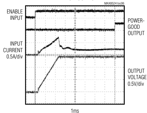
SOFT-START WAVEFORMS AT 1.45V OUTPUT
