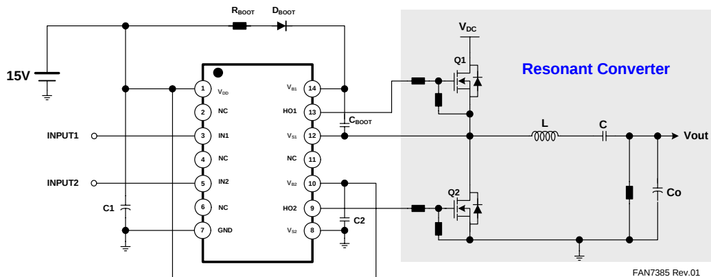
Figure 3. Half-Bridge LCC Resonant Converter Application
