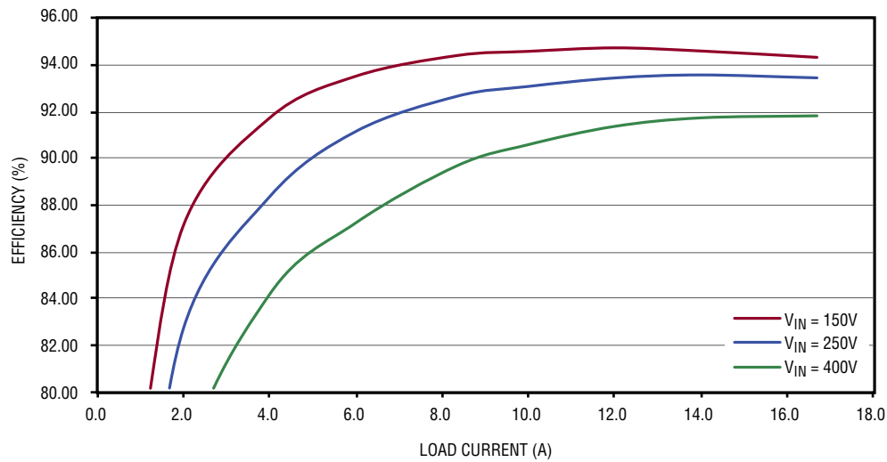
Figure 3. Typical Efficiency Curve, (300LFM, TA = 25°C)
