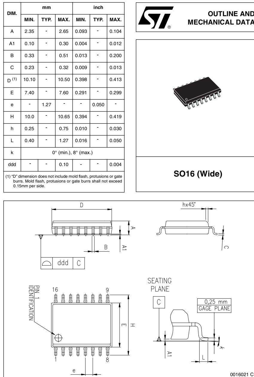
Figure 13. SO16 (Wide) mechanical data and package dimensions
