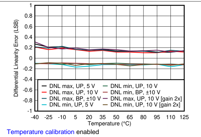
Figure 6. Differential Linearity Error vs Temperature
