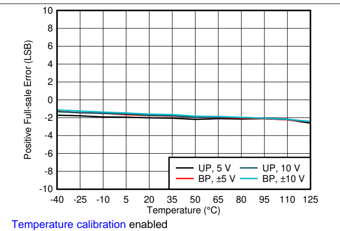
Figure 8. Positive Full-Scale Error vs Temperature
