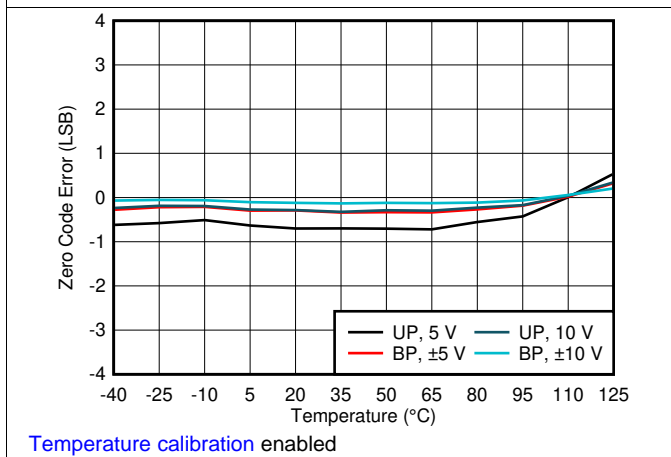
Figure 7. Zero Code Error vs Temperature
