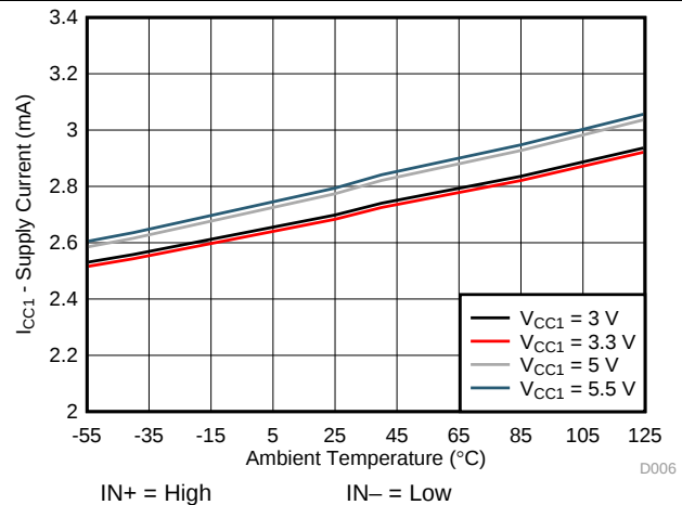
Figure 19. I_{CC1} Supply Current vs Temperature
