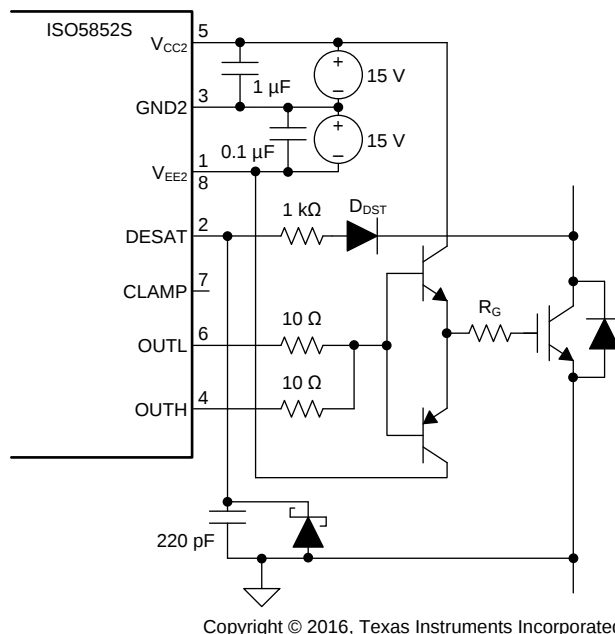
Figure 57. Current Buffer for Increased Drive Current
