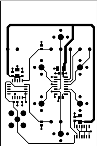
Component Side
