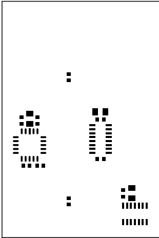
Paste Mask Top
