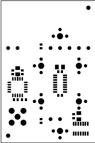
Component Side Solder Mask
