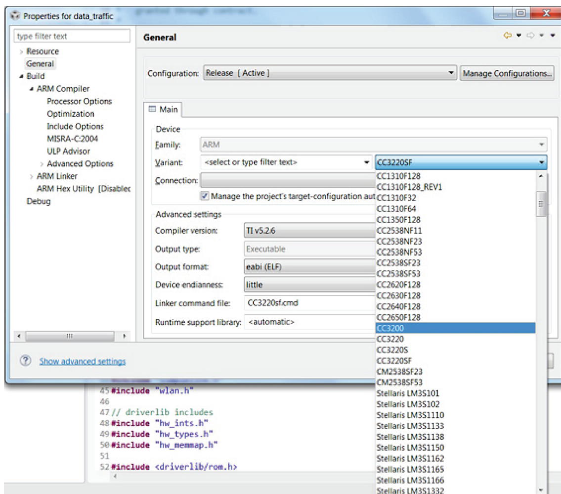
Figure 2-4. Select Device Variant
