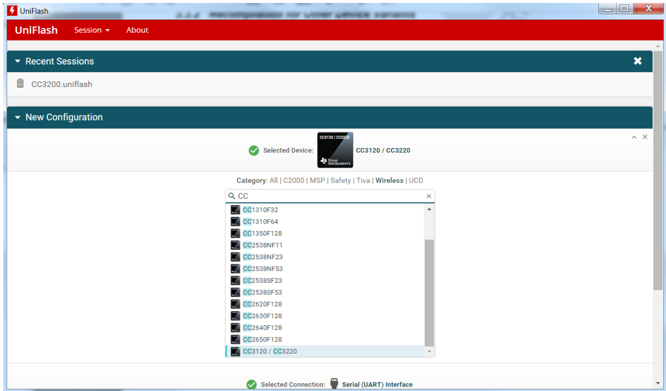
Figure 2-5. UniFlash – Select Device
