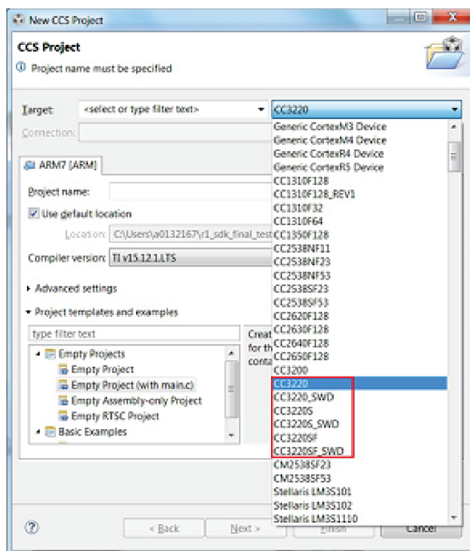
Figure 1-12. Device Variant for CCS
