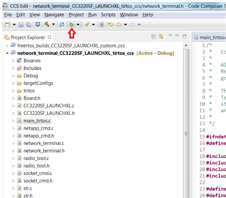
Figure 3-5. Debug Network Terminal
