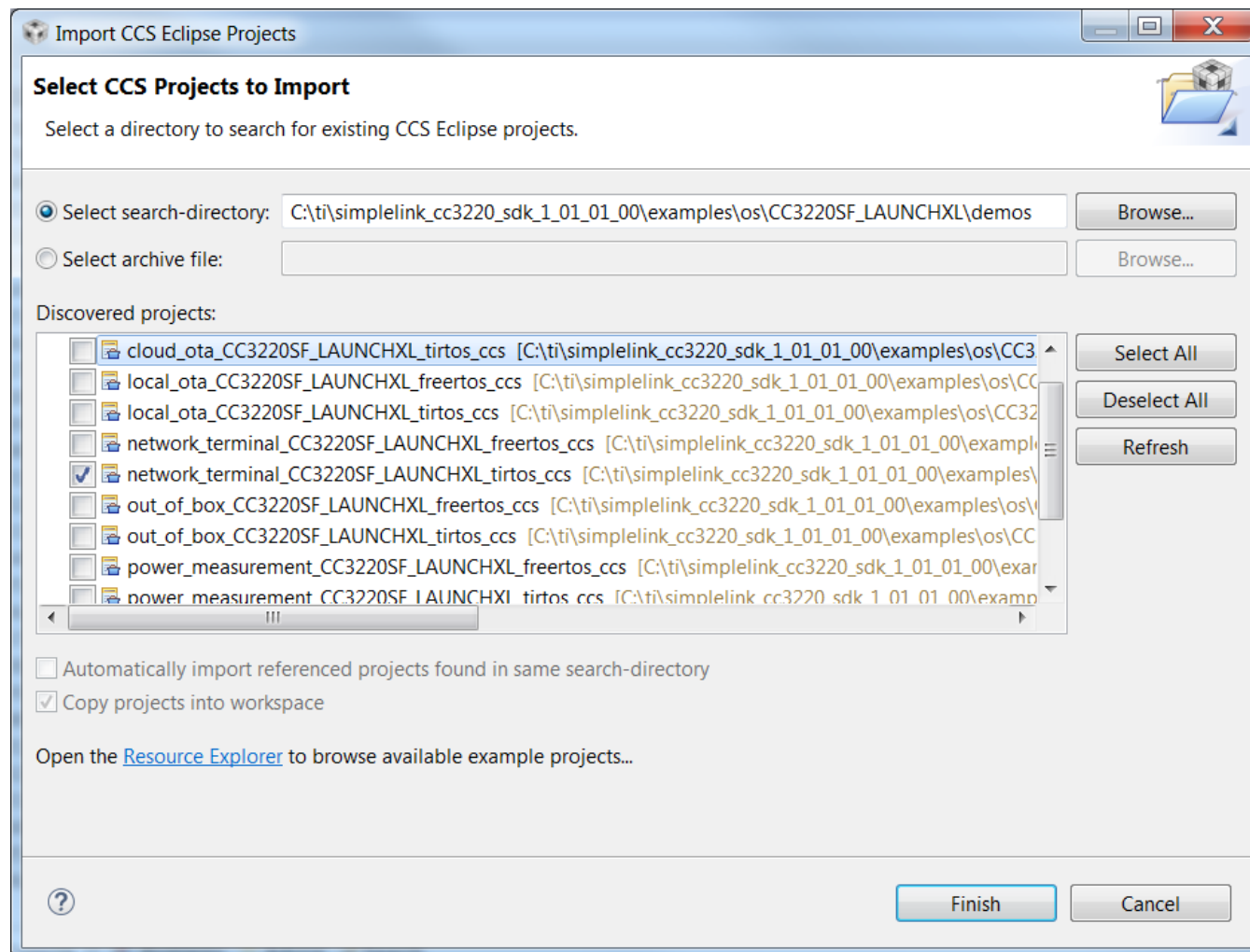
Figure 2-2. Select wlan_station Projects
