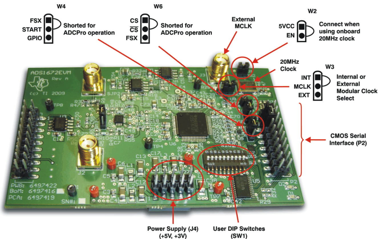
Figure 4. Digital Interface Connectors and Jumpers
