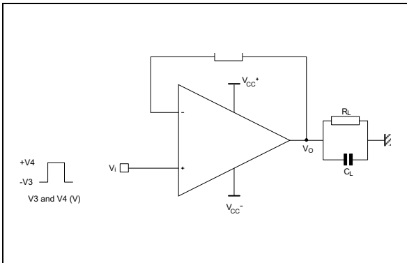
Figure 3 : Slew Rate
