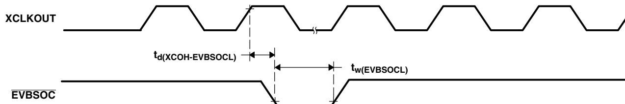
Figure 6–18. EVBSOC Timing
