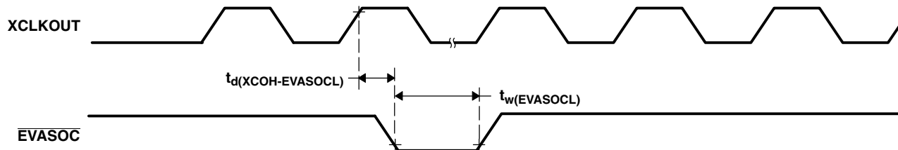
Figure 6–17. EVASOC Timing
