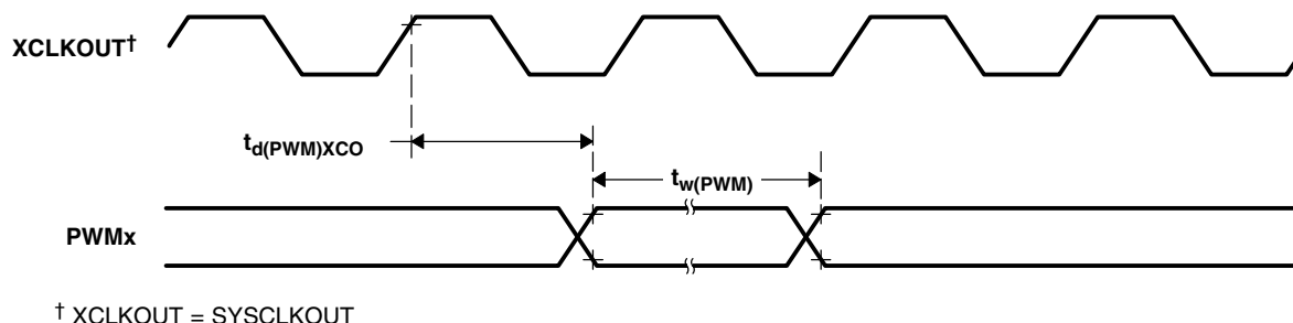
Figure 6–15. PWM Output Timing
