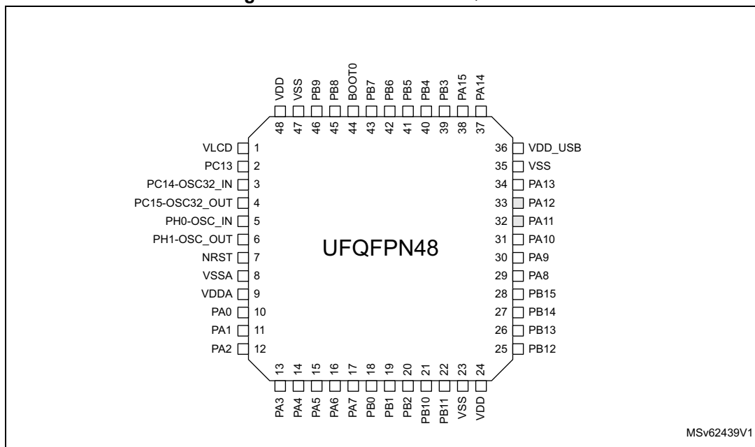
Figure 8. STM32L073xx UFQFPN48
