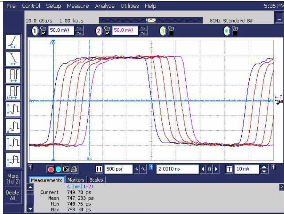
Delays from 0 to 2250 ps on CLKout1 referenced to CLKout0
