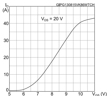
Figure 5: Transfer characteristics
