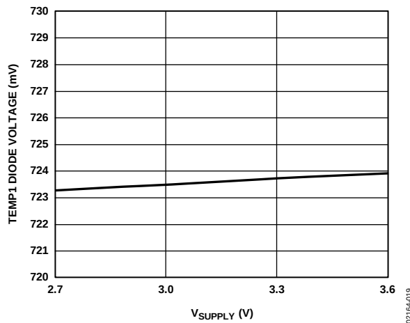
Figure 19. TEMP1 Diode Voltage vs. V_{SUPPLY} (25 ^{\circ} C)
