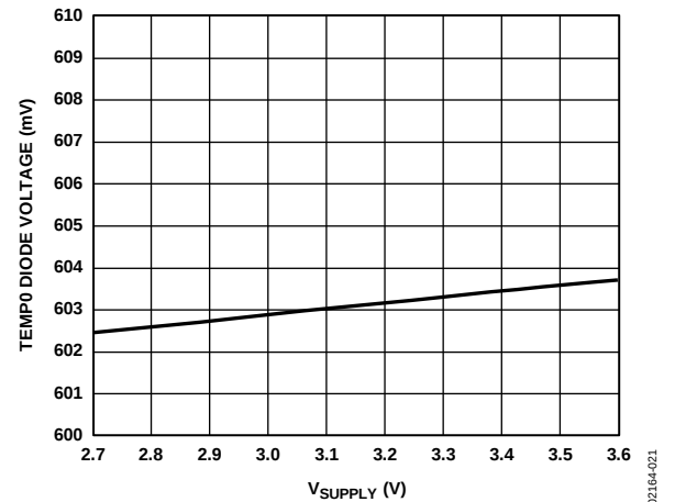
Figure 21. TEMP0 Diode Voltage vs. V_{SUPPLY} (25 ^{\circ} C)
